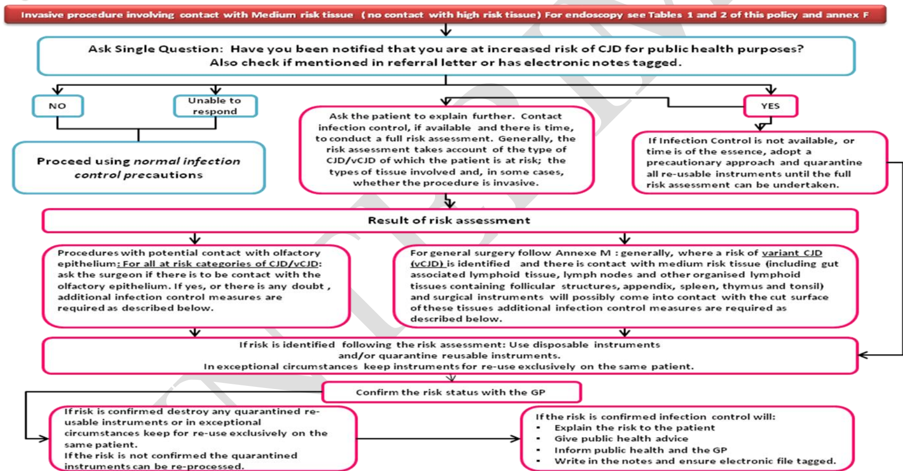
CJD Algorithm 1
